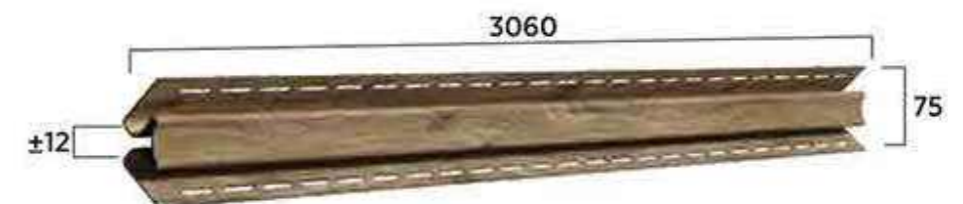
Inside Corner Profile
